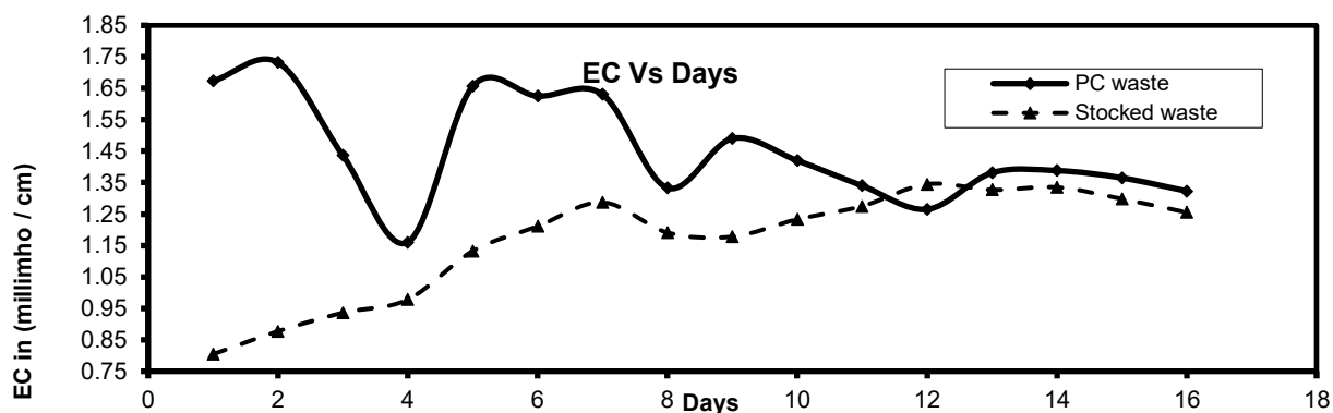
Fig. 4 EC Vs days
