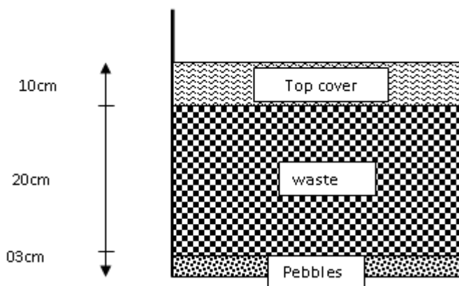
Fig.2 Vermi bin
