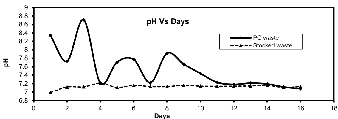
Fig.3 pH Vs days
