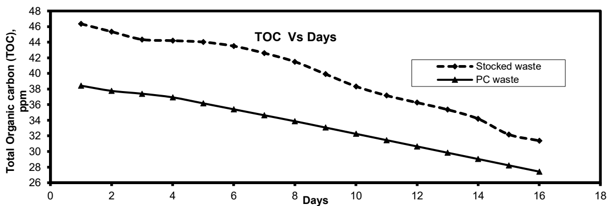
Fig. 5 TOC Vs days
